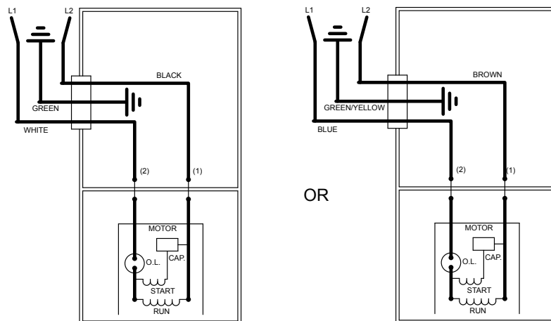
WIRING DIAGRAM FOR MODELS "V98-A," "V98-B," "V98-C" 11/90 thru Current 009059
