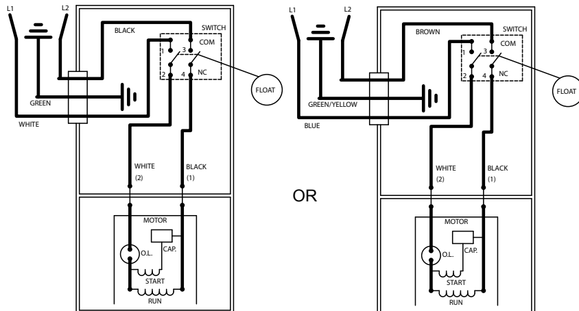
WIRING DIAGRAM FOR MODELS "U98-A," "U98-B," "U98-C" 11/90 thru Current 009060
