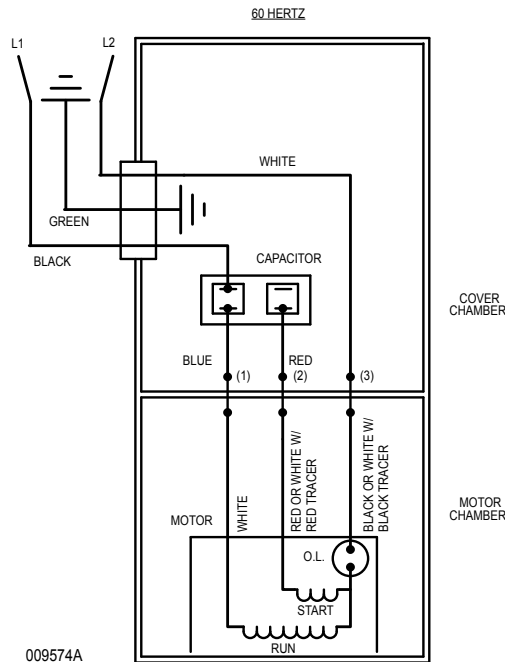
WIRING DIAGRAM FOR MODELS "N140" All Revisions; "N4140" All Revisions; "E140" All Revisions; "E4140" All Revisions 2/95 thru Current
